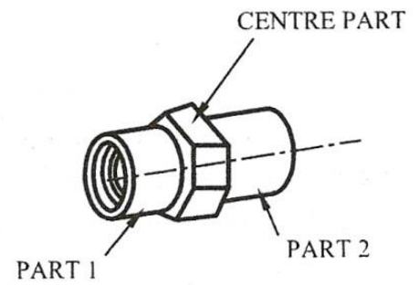
UNION
